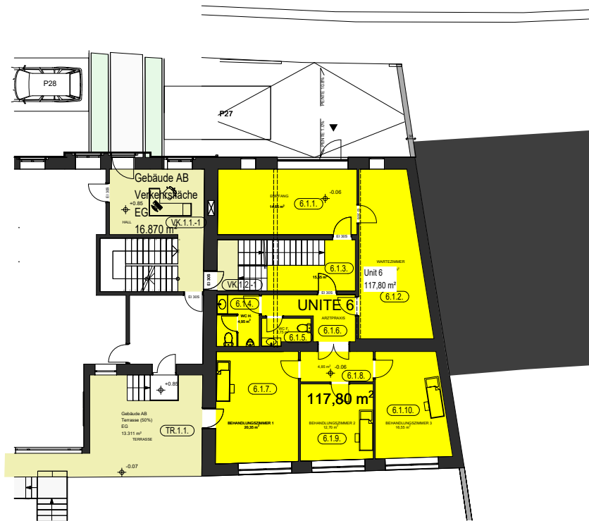
Grundriss Erdgeschoss (Unit 6)
